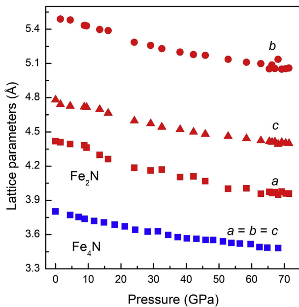
Fig. 4. The lattice parameters of \text{Fe}_2\text{N} and \text{Fe}_4\text{N} as a function of pressure. The error bars are smaller than the symbols.
