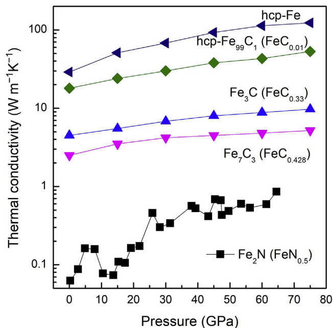
Fig. 8. The pressure-dependent thermal conductivity of \text{Fe}_2\text{N} . The data were converted from relative electrical conductivity using Wiedemann-Franz law at 300 K. The symbols are the same as Fig. 7. The error bars are smaller than the symbols.
