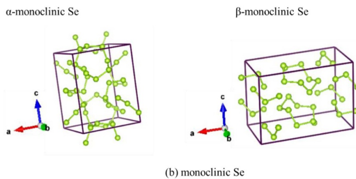
Figure 3. Schematics of Se atomic configurations in various states.
