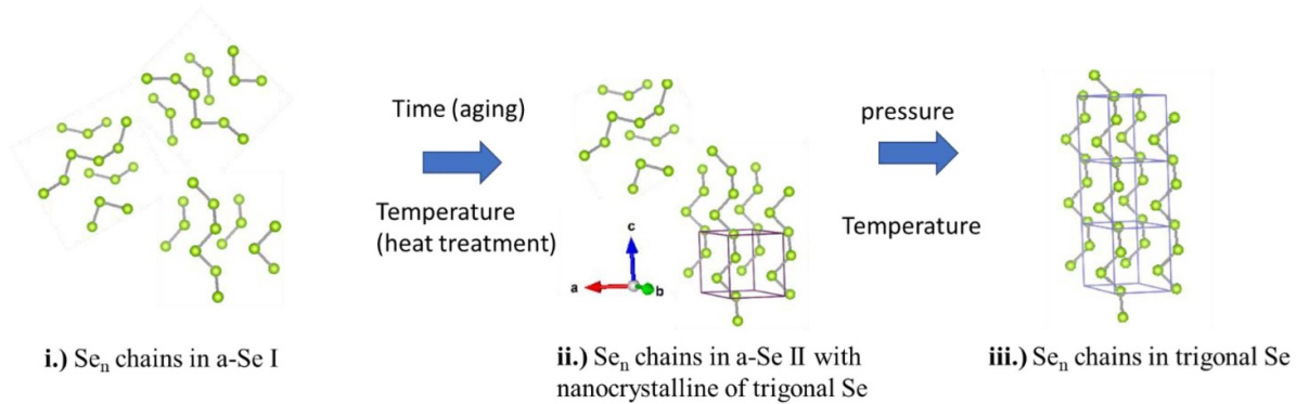
(a) Helical \text{Se}_n chains in i.) fresh amorphous state a-Se I, ii.) aged amorphous state a-Se II, iii.) trigonal Se.
