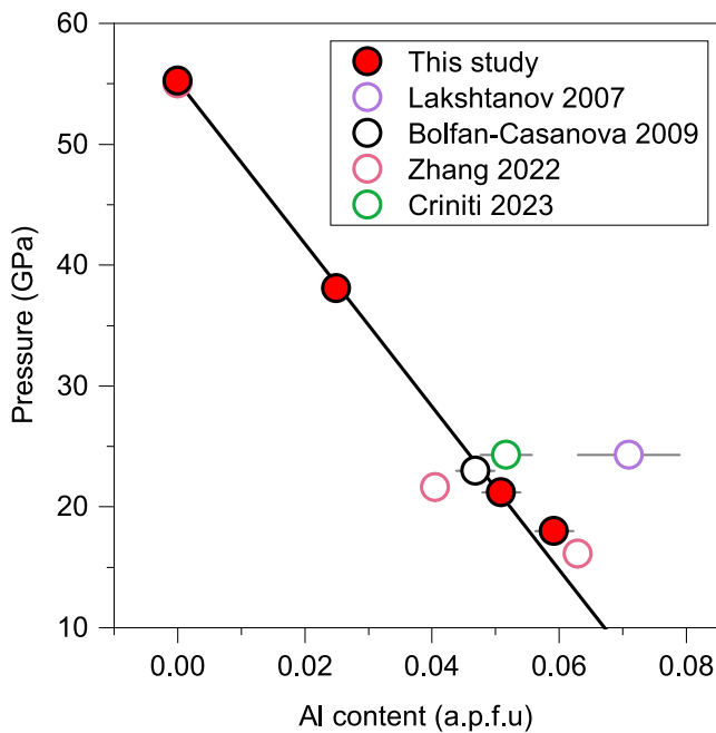
Figure 2. The effect of Al content on the post-stishovite transition pressure at 300 K. Red: this study; purple: Lakshtanov, Sinogeikin, et al. (2007); black: Bolfan-Casanova et al. (2009); pink: Zhang et al. (2022); green: Criniti et al. (2023). Solid line: the transition pressure as a function of Al content when the H/Al ratio in stishovite is \sim 1/3 ; Error bars smaller than the symbols are not shown.
