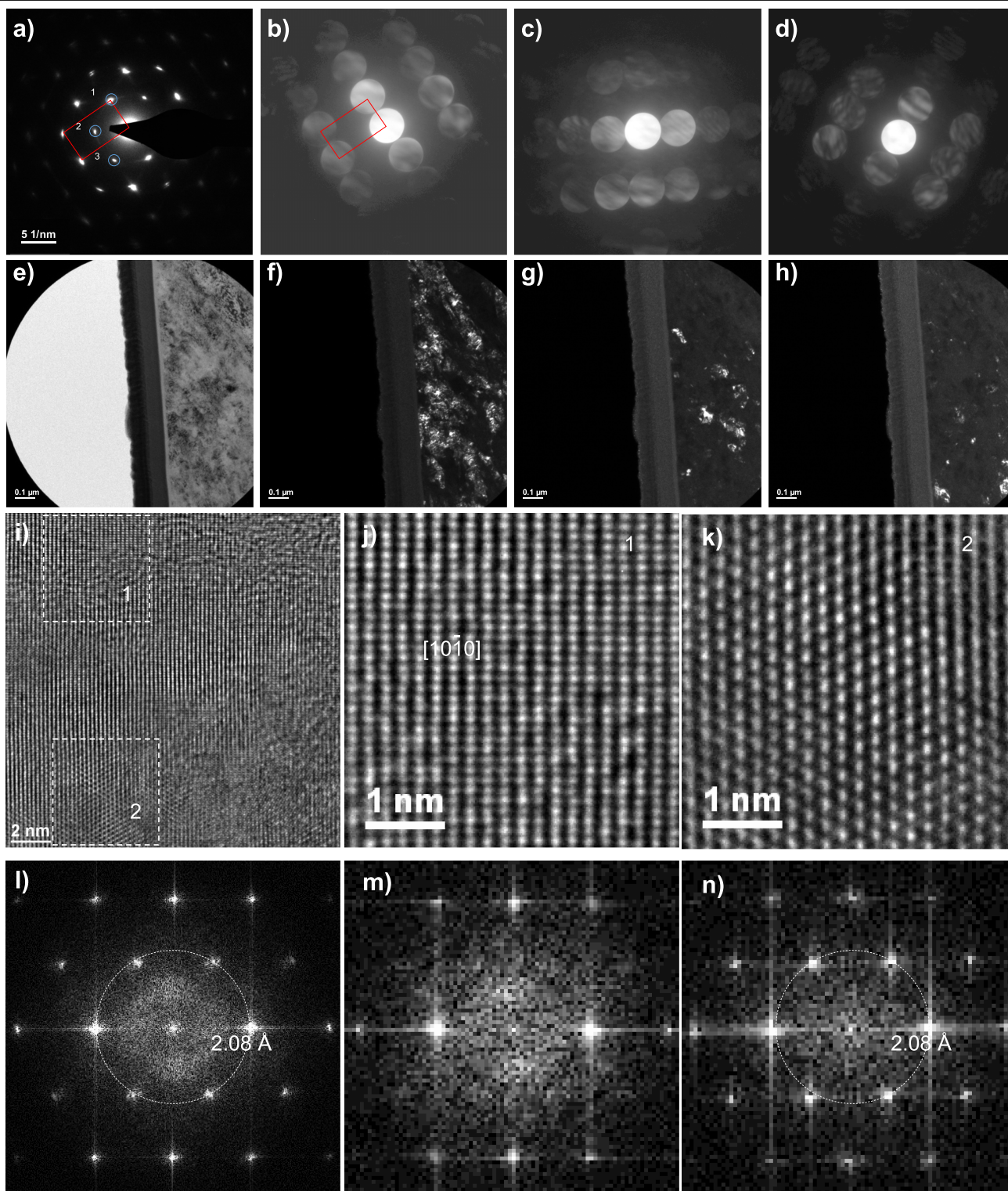
Extended Data Fig. 3 | TEM study of the microstructure in triple twinned HD domains. a , SAD pattern using a large, selected-area aperture. b–d , Convergent electron diffraction patterns showing three sets of diffraction patterns from each set of triple-twinned domain. Each variant has a twofold [10\bar{1}0] diffraction pattern separated by 120^\circ . e , Bright-field TEM image showing triple-twinned microstructure in our high P - T synthesized HD. f–h , Dark-field images using diffraction spots 1, 2 and 3 marked in a show that there exist three variants. i , A large-area HRTEM
