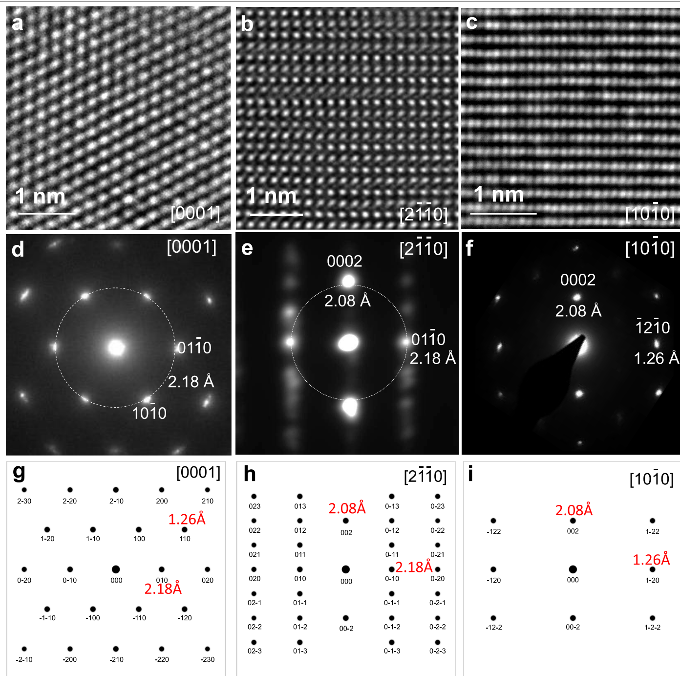
Extended Data Fig. 5 | HRTEM and electron diffraction patterns of HD from three major zone axes. a–i, HRTEM images (a–c), corresponding SAD patterns (d–f) and simulated electron diffraction patterns (g–i) from three main zone axes [0001] , [2\bar{1}\bar{1}0] and [10\bar{1}0] , respectively.
