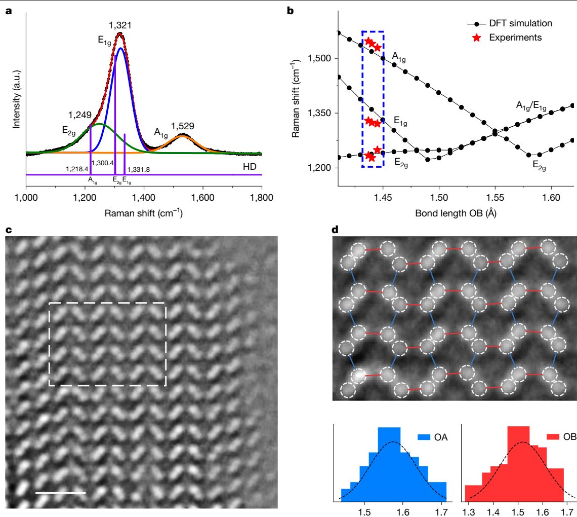
Fig. 3 | The two distinct bond lengths characteristic of HD were determined through complementary techniques: UV Raman spectroscopy, simulated Raman spectra and AC-HRTEM. a , UV Raman spectrum of the recovered HD sample showing three peaks (1,249, 1,321 and 1,529 cm -1 ), marked by different colours. The bottom purple Raman spectrum is calculated on the basis of an ideal HD structure (ref. 24). b , Calculated Raman spectra of HD based on bond length OB shows three Raman modes (A 1g , E 1g and E 2g ). Experimentally observed
