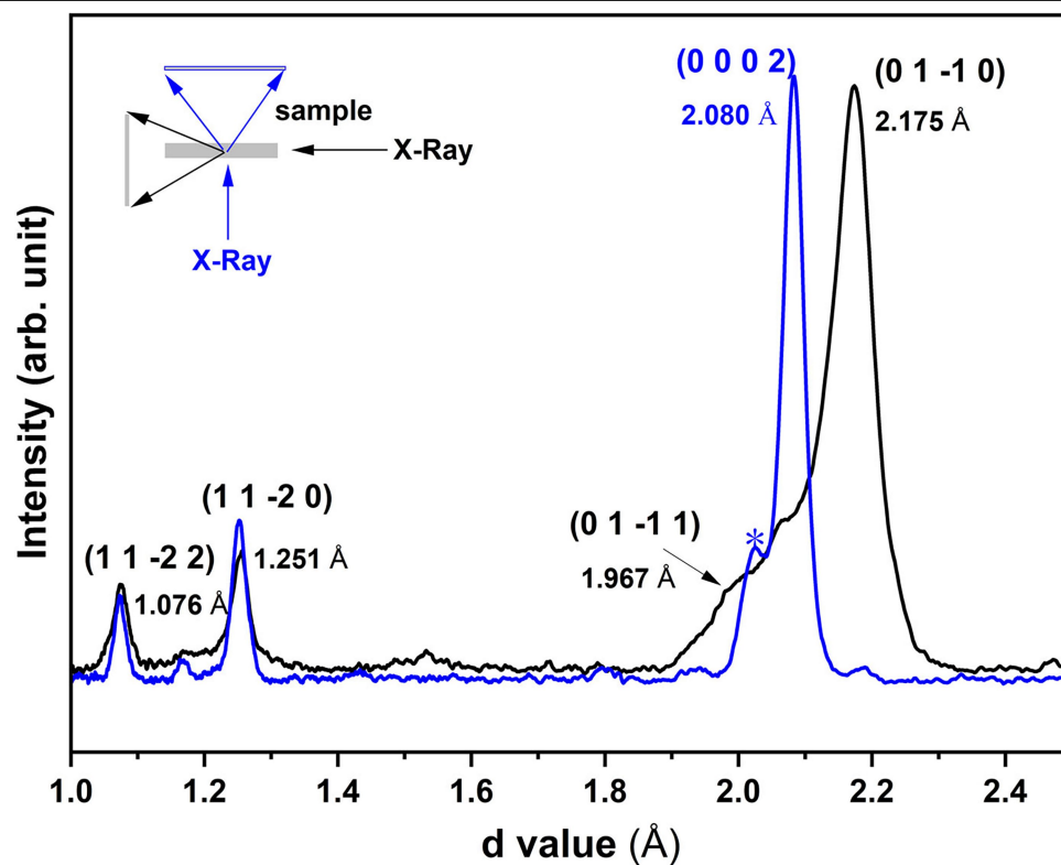
Extended Data Fig. 2 | The integrated XRD patterns from the recovered HD sample with incident X-ray beam along (blue) and perpendicular to (black) the c-axis of starting graphite crystal. The weak diffraction ring marked with
