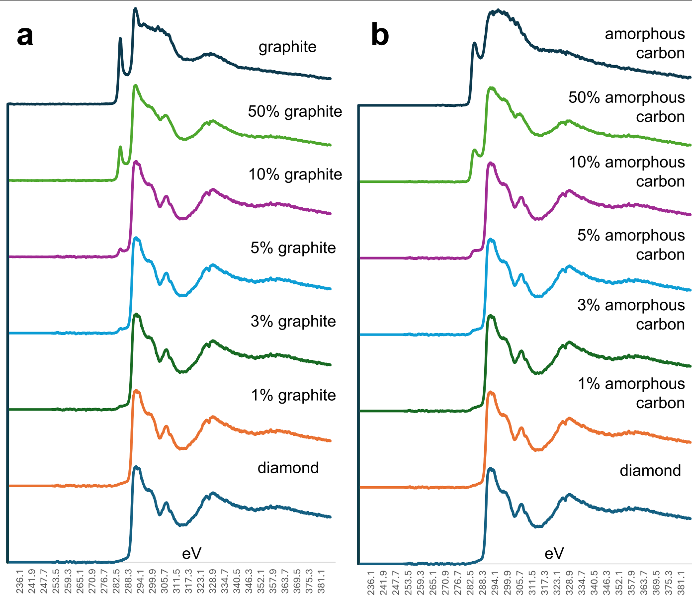
Extended Data Fig. 9 | EELS spectra from the mixture of different polytypes of carbon. a, EELS spectra summed from diamond and graphite with different percentages. b, EELS spectra summed from diamond and amorphous carbon
