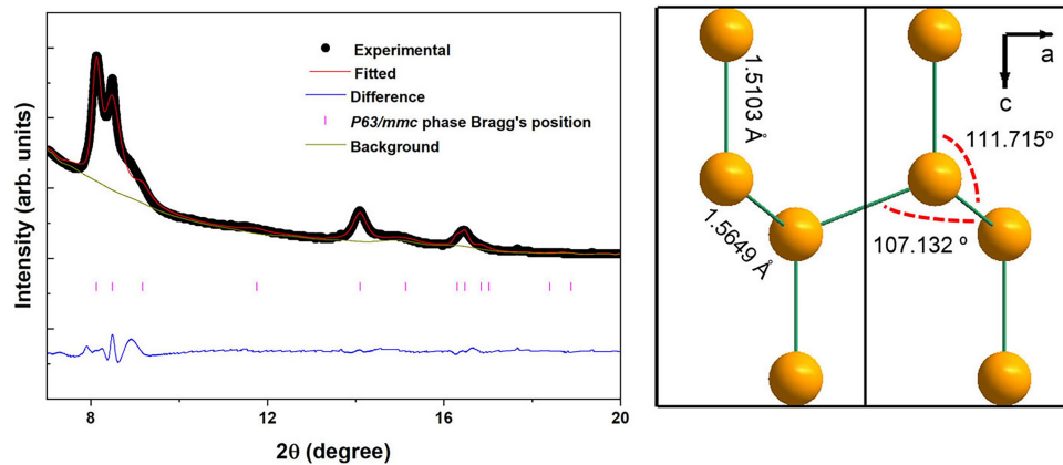
Extended Data Fig. 7 | Rietveld refinement on the integrated XRD pattern from a recovered HD sample with lattice constants a=b=2.5182 Å and c=4.1780 Å. The right panel presents the atom arrangement with two sets of bond length (1.5103 Å and 1.5649 Å) and two sets of bond angle (107.132° and 111.715°).
