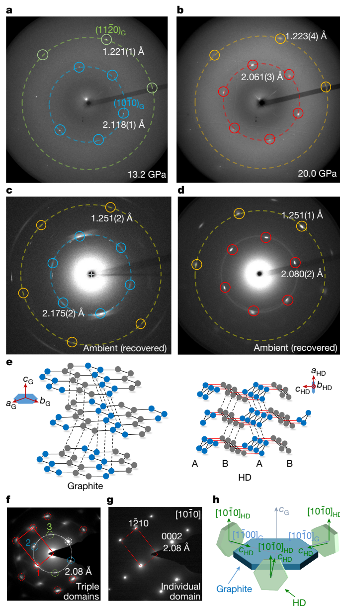
Fig. 1 | Single-crystal phase transition from graphite to HD under high pressure and high temperature and their epitaxial crystallographic relationship. a, b , Near-c-axis XRD pattern on graphite sample taken at 13.2 and 20.0 GPa. c, d , XRD patterns of recovered HD sample after laser heating to 1,400 °C at 20.0 GPa taken with incident X-ray perpendicular and parallel to the c -axis of the starting graphite sample. The diffraction spots in a, b and d all show a clear hexagonal symmetry. e , The atomic transformation from graphite to HD. Black solid and dashed lines connecting spheres of the same colours form new honeycombs of HD and red lines on the c -axis form bonds between HD honeycombs. Blue and black spheres represent the close-packed planes of HD in the ABAB stacking sequence. f , SAD pattern of the recovered specimen from a large area (1 \mu m in diameter) showing a hexagonal-like pattern, similar to the XRD result in d . g , SAD pattern from a 200-nm area showing a twofold symmetry that can be well indexed by HD [10 \bar{1} 0] zone axis pattern of a single nanocrystal. h , Schematic of the epitaxial relationship between graphite and HD.
