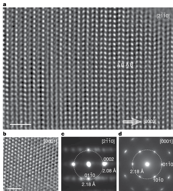
Fig. 2 | HRTEM images and corresponding SAD patterns of the bulk HD sample were acquired along different zone axes. a, b, HRTEM images along HD [2 \bar{1} 10] and [0001] zone axes showing a large area of HD with AB stacking and honeycomb configuration, respectively. Scale bars, 1 nm. c, d, SAD pattern along [2 \bar{1} 10] and [0001] using a 200-nm selected-area aperture. c, Extinction of (0001) diffraction owing to strict AB stacking. d, SAD along HD [0001] showing hexagonal diffraction spots with a d -value of 2.18 Å.
