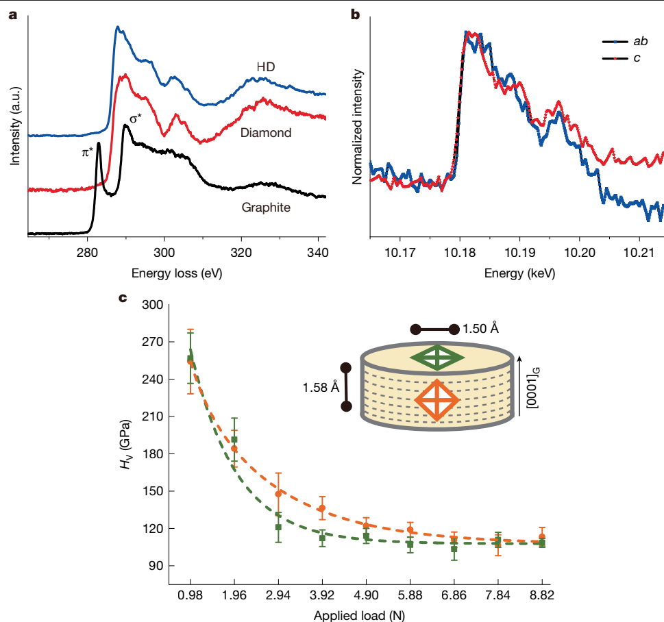
Fig. 4 | Pure sp^3 bonding state and the excellent mechanical properties of bulk HD. a , EELS spectra of carbon k-edge from HD, diamond and graphite. b , X-ray Raman spectra on recovered HD samples with ab and c orientation. All results indicate 100% sp^3 bonding in the HD. c , Vickers hardness tests of HD along two directions with different load (N) up to 8.8 N. Inset, schematic of the
