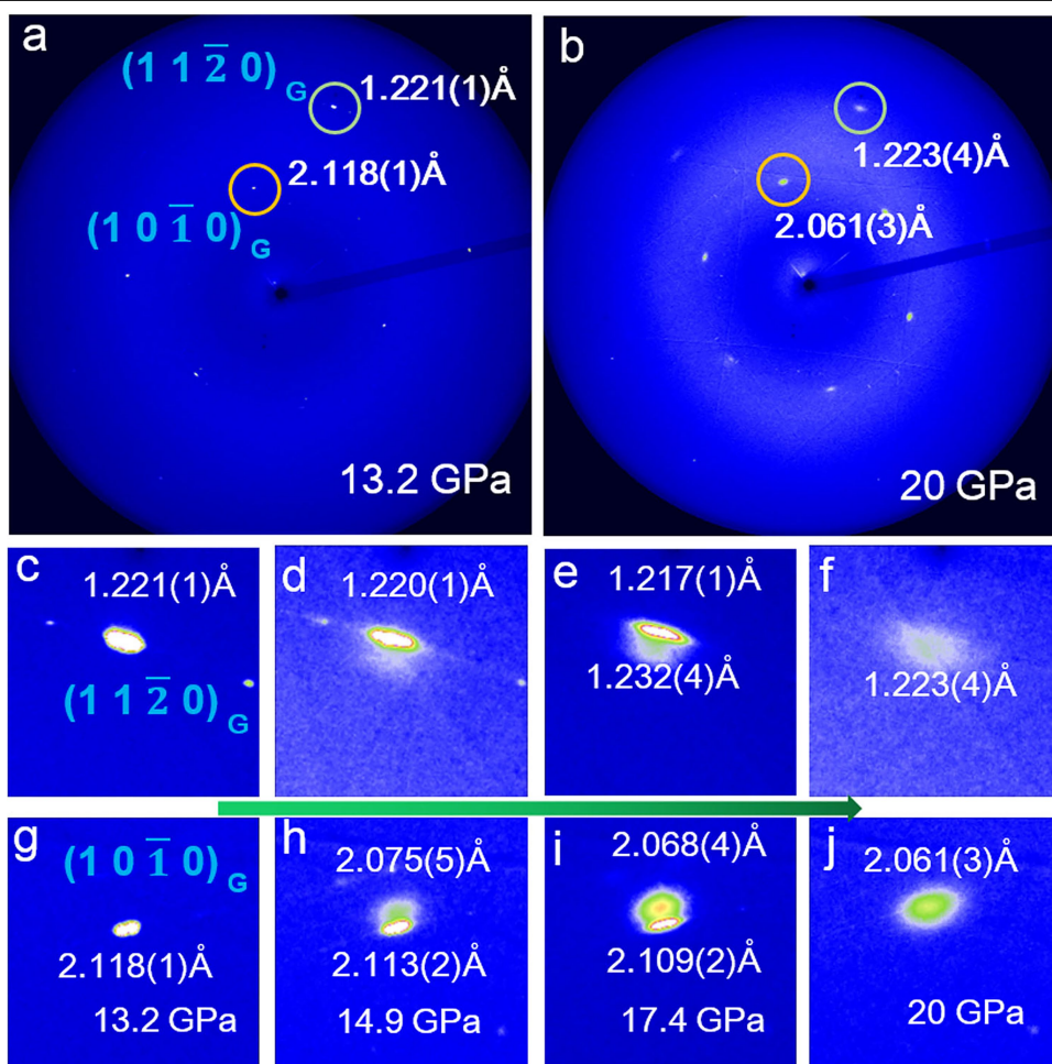
Extended Data Fig. 1 | XRD images of hexagonal graphite at different pressures before and after transition. a, 13.2 GPa. b, 20.0 GPa. The incident X-ray beam is parallel to the c -axis of pristine graphite. The graphite (10\bar{1}0) and (11\bar{2}0) diffraction spots at 13.2 GPa and the corresponding spots appearing at 20.0 GPa are labelled by orange and green circles in a and b , respectively. c–j , Evolution of the (11\bar{2}0) and (10\bar{1}0) diffraction spots under pressures between
