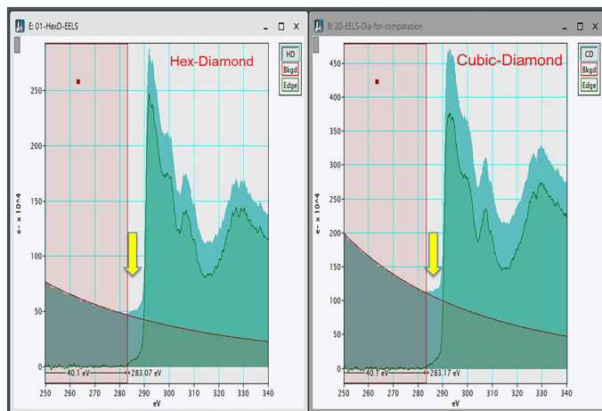
Extended Data Fig. 8 | EELS spectra from HD and cubic diamond. A very small pre-peak indicated by the yellow arrow in the HD EELS spectra can be seen. The estimated sp^2/sp^3 is around 3%, resulting from the amorphous surface layer owing to FIB sample preparation.
