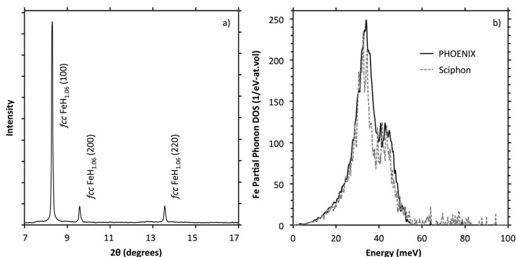
Figure 1. (a) Measurements of quenched nonstoichiometric ( X \sim 1.06 ) fcc \text{FeH}_x at 64 GPa, including (a) Integrated X-ray diffraction with \text{FeH}_x peaks are labeled with their respective Miller indices, and (b) Fe partial phonon density of states (DOS). The DOS indicated by the solid black line was obtained using the PHOENIX program (Sturhahn, 2000), and dotted grey line is the DOS obtained from Sciphon 1.0.3 (Dauphas et al., 2014).
