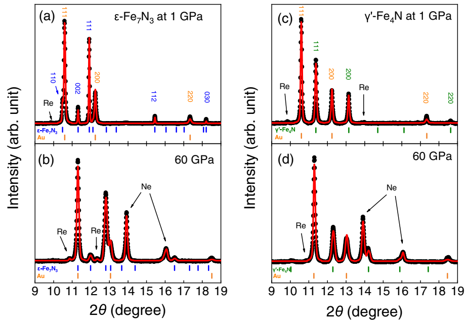
Figure 1. Panels (a) and (b) are representative X-ray diffraction patterns of \epsilon -Fe 7 N 3 at 1 and 60 GPa at 300 K, respectively; panels (c) and (d) are representative X-ray diffraction patterns of \gamma' -Fe 4 N at 1 and 60 GPa at 300 K, respectively. Le Bail refinements (red solid curves) of observed XRD data (black dots) were carried out after background subtraction, demonstrating all sample peaks match hexagonal \epsilon -Fe 7 N 3 and cubic \gamma' -Fe 4 N, respectively, within the investigated pressure range. The vertical ticks are \epsilon -Fe 7 N 3 (blue), \gamma' -Fe 4 N (dark green), and the pressure calibrant, Au (orange). The wavelength of the incident X-ray beam was 0.434 Å.
