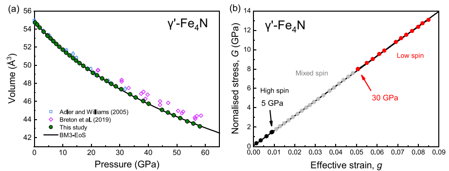
Figure 4. Compression behavior of \gamma' -Fe 4 N at 300 K. (a) Unit-cell volume of \gamma' -Fe 4 N up to 60 GPa at 300 K determined from X-ray diffraction measurements in this work (dark green circles), together with previous experimental results. The black curve represents the third-order Birch-Murnaghan equation of state (BM-EoS) fit of all pressure-volume data from this study. (b) Normalized stress G as a function of effective strain g . Solid black, gray, and red circles represent the results of high-spin, mixed-spin, and low-spin state, respectively, as determined by XES. The black solid line indicates a linear fit for all data. The pressure of onset and completion of spin transition is indicated by XES, but no change in compressibility can be observed in either plot.
