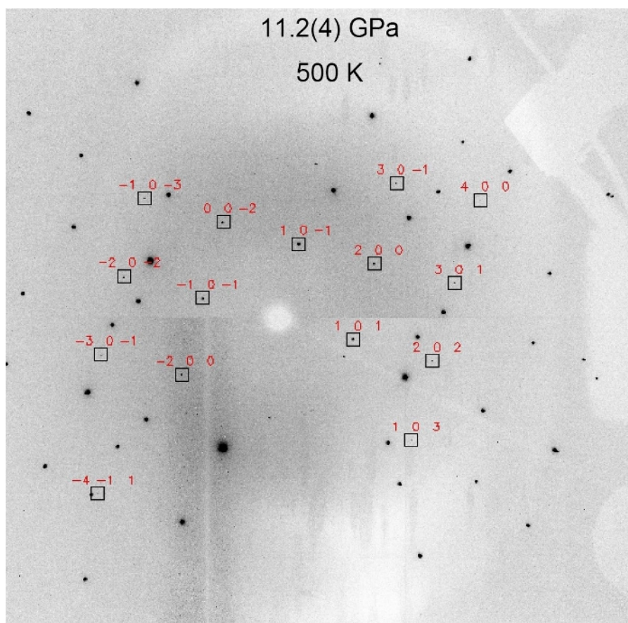
Figure 5: Single crystal XRD pattern of ice-VII at 11.2 GPa and 500 K.
