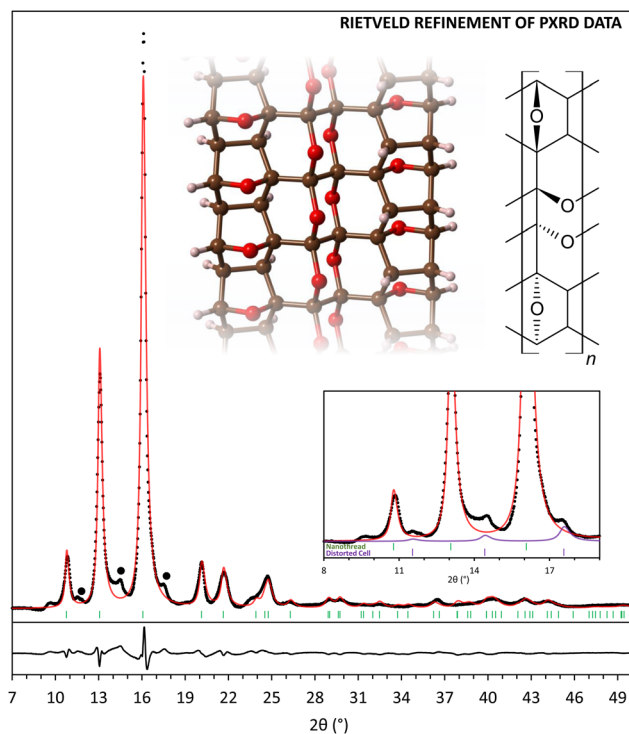
Fig. 3 X-ray diffraction pattern ( \lambda = 1.541 \text{ \AA} ) of \alpha -furil nanothreads synthesized in a Paris-Edinburgh press and recovered to 1 atm (black points) with Rietveld refinement using nanothread structure C (red line). Black dots indicate peaks corresponding to unidentified phases. Inset, top: A segment of refined nanothread structure C and associated structural formula. Inset, bottom: X-ray diffraction pattern of \alpha -furil nanothreads between 8 and 19°. Green tick marks indicate the relative positions of the three low-angle reflections for the refined nanothread polymer. Purple pattern and tick marks indicate the relative positions of the three low-angle reflections for an expanded lattice of phase II \alpha -furil.
