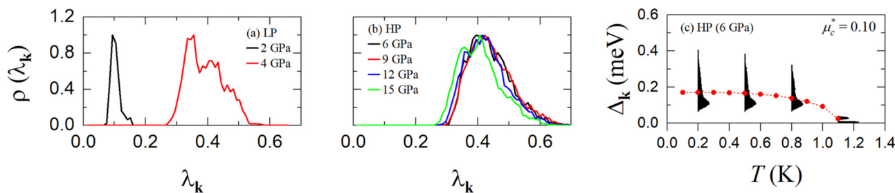
Fig. 9 Distribution of the e-ph coupling strength \lambda_{\mathbf{k}} of (a) the LP and (b) the HP phase of AuAgTe 4 at various pressures. (c) Energy distribution of the anisotropic superconducting gap \Delta_{\mathbf{k}} of the HP phase as a function of temperature at 6 GPa. The red symbols represent the isotropic superconducting gap at 6 GPa. The Coulomb parameter is set to \mu_c^* = 0.10 .
